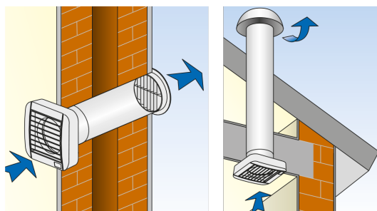
Wandmontage
